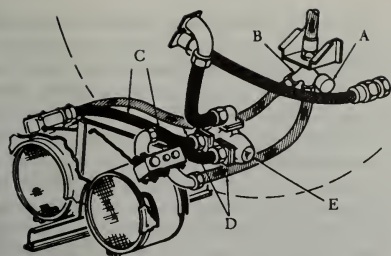
FIGURE 6-8. Dual oil cooler system.
